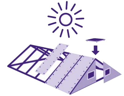
4. Attach panels, ventilation and solar panel
